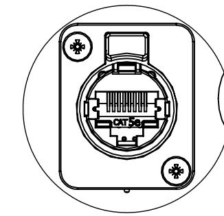
DETAIL A OPTION 1 GX CONNECTOR RJ45, CAT5E
