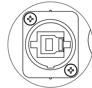
DETAIL A OPTION 2 U CONNECTOR USB 3.0, TYPE B
